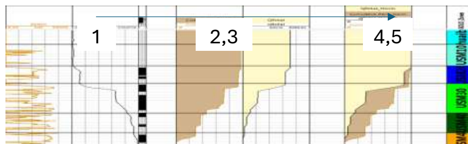
Figure 2. Process the log permeability and ILT inflow in the units of Zubair Formation
