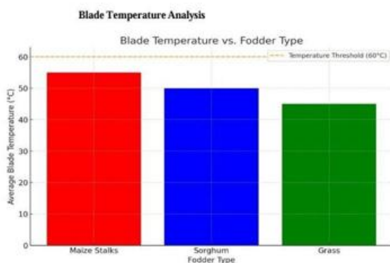
Fig. 5. Blade Temperature Analysis
