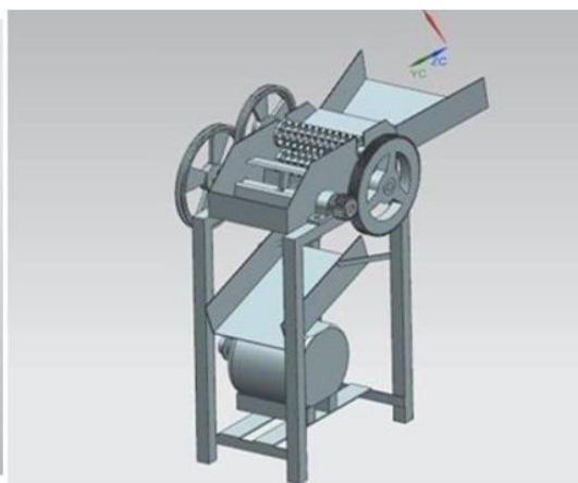
Fig. 2. Full Drawing Model
