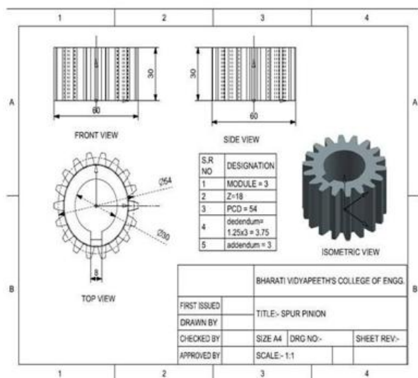
Fig.3 Spur Gear
