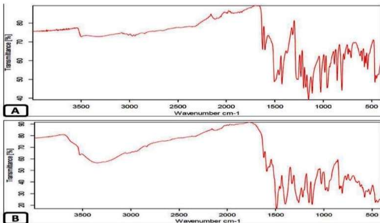
Figure 2. FTIR spectra of (A) Hedychium coronarium and (B) Zinc- Hedychium coronarium complex.
