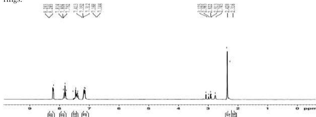
Figure 3. ^1\text{H} -NMR spectra of Zinc- Hedychium coronarium complex.
