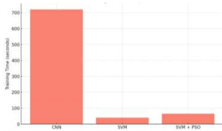
Fig. 3. Model Comparison using Training Time
