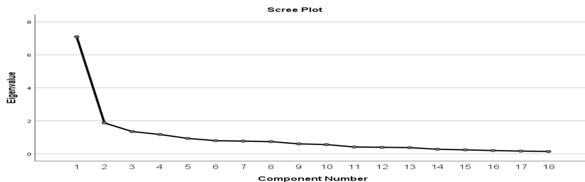
Chart 1: Scree Plot
