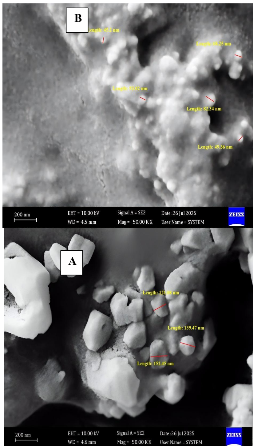
Figure (17). Scanning Electron Microscopy (SEM) micrographs of the Gel/PEG/ZnO polymer matrix at 200 nm magnification: (A) prior to drug loading (B) after drug loading
