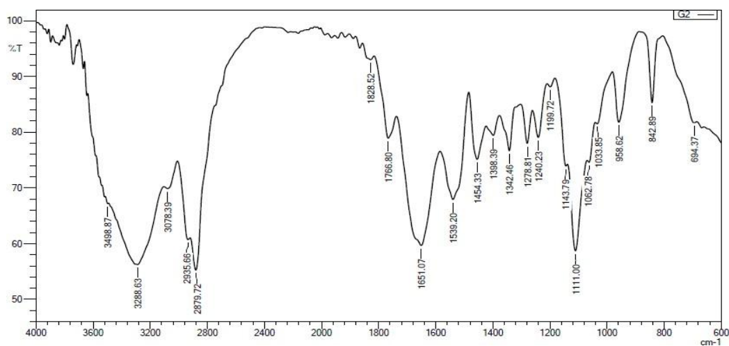
Figure (2) FTIR spectrum of the Gel/PEG/ZnO hydrogel matrix after cephalexin loading.
