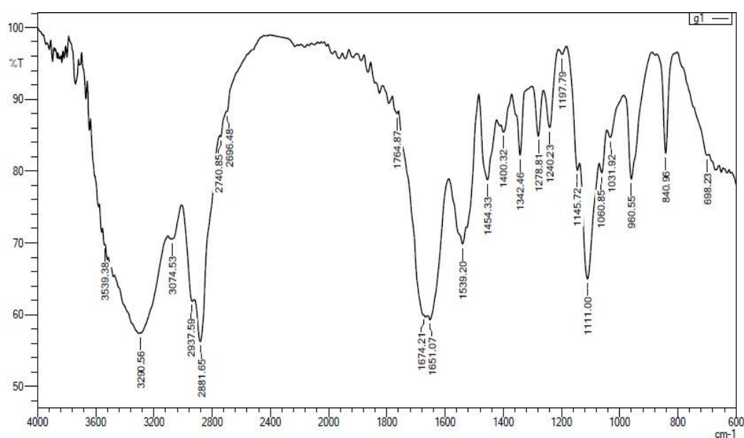
Figure (1) FTIR spectrum of the Gel /PEG/ZnO hydrogel matrix before cephalexin loading
