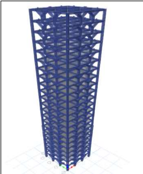
Figure 9: Rendered View of Model 1: G+20 Storied RC Structure with Y-shaped Columns
