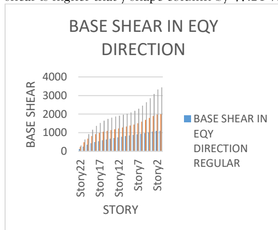
Graph 6-Base Shear in EQY Direction
