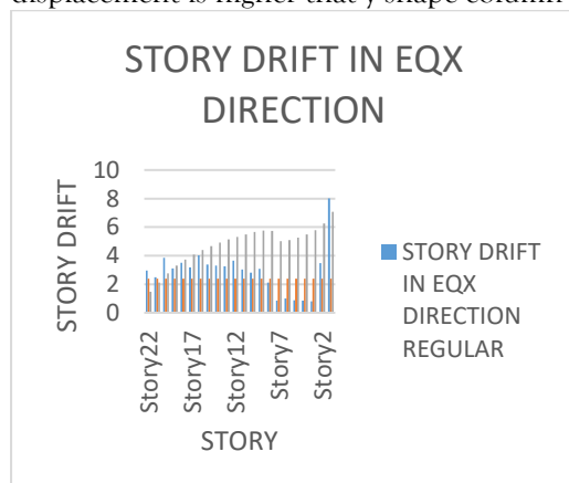
Graph no 3- Story Drift in EQX Direction
