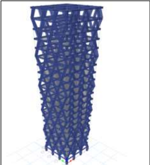
Figure 8: Rendered View of Model 1: G+20 Storied RC Structure with Oblique Columns • Model 2: G + 20 Storied RC Structure with Y-shaped Columns
