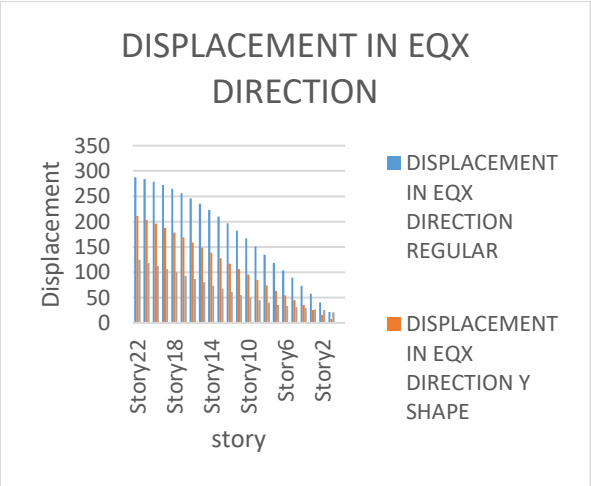
Graph no 1- Displacement in EQX Direction
