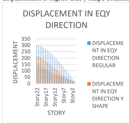
Graph no 2- Displacement In EQY Direction
