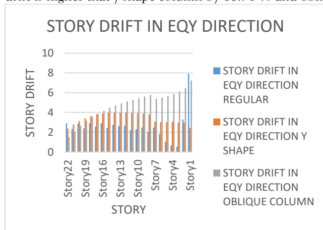
Graph no 4 Story Drift In EQY Direction
