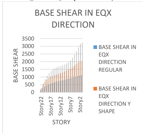
Graph no 5- Base Shear in EQX Direction
