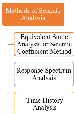
Figure 5: Methods of Seismic Analysis
