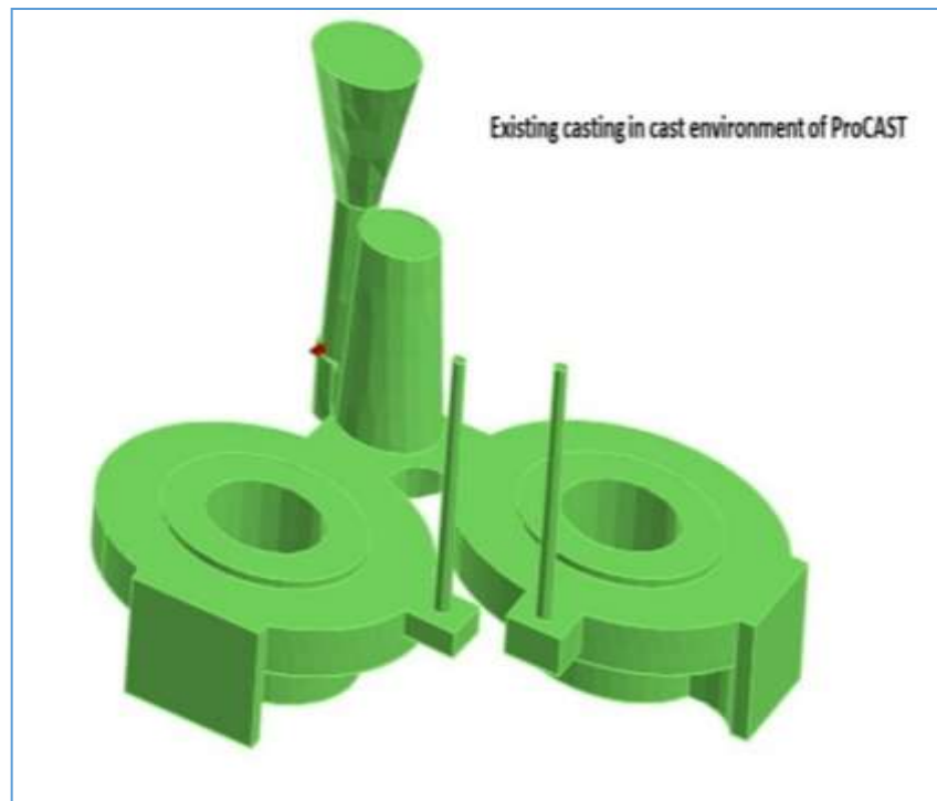
Figure 4 Existing CAD model in ProCAST environment
