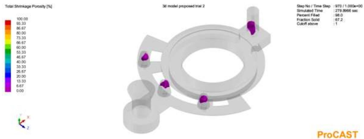
Figure 16 Shrinkage porosity
