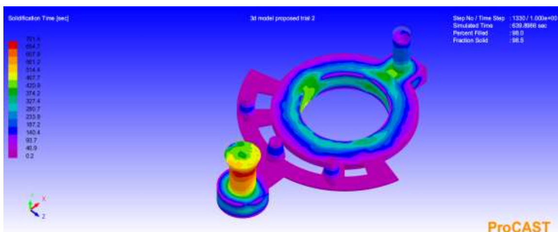
Figure 14 solidification time
