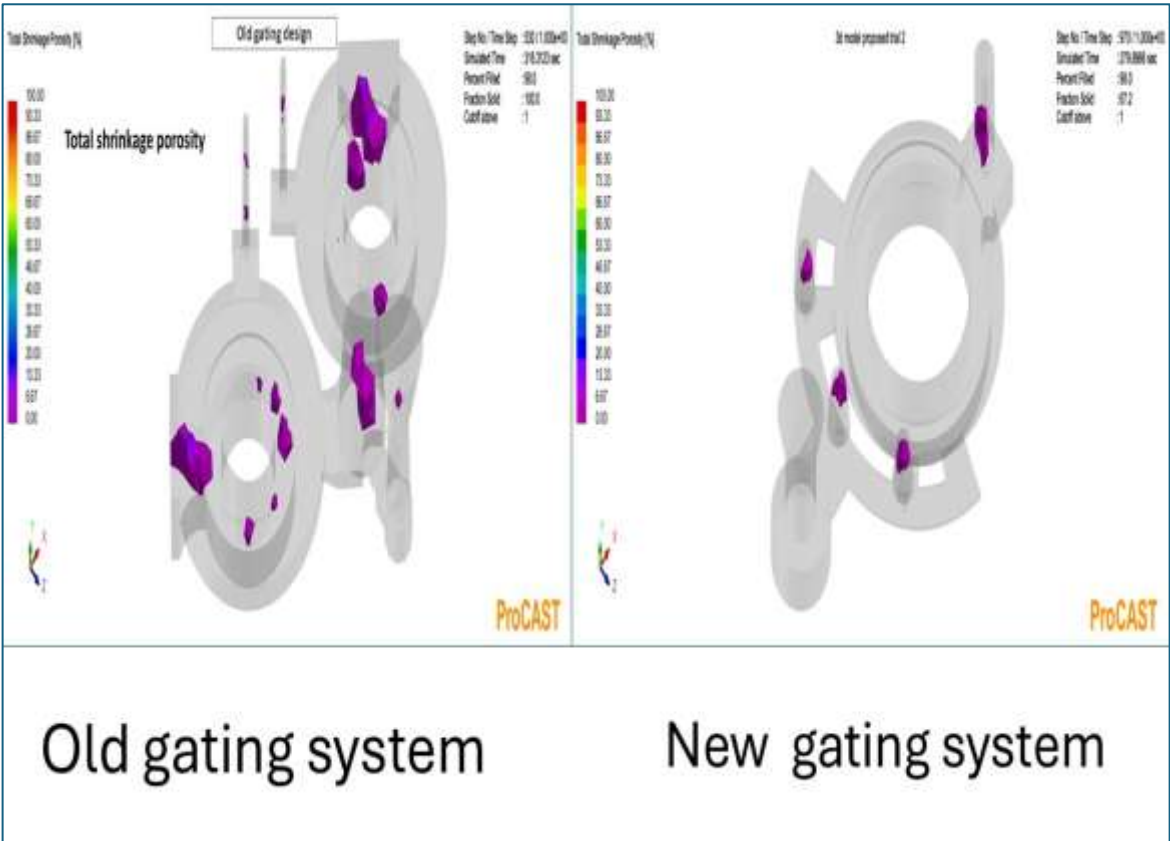
Figure 19 Comparison of simulation results
