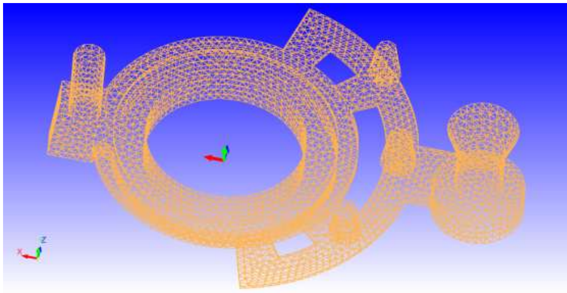
Figure 12 3D geometry of meshed valve body
