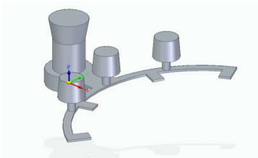
Figure 7 Proposed feeders and gating system
