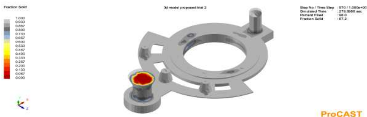
Figure 15 Fraction of solid
