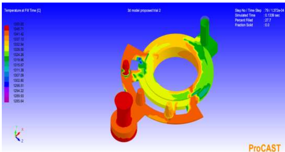
Figure 13 Temperature at fill time
