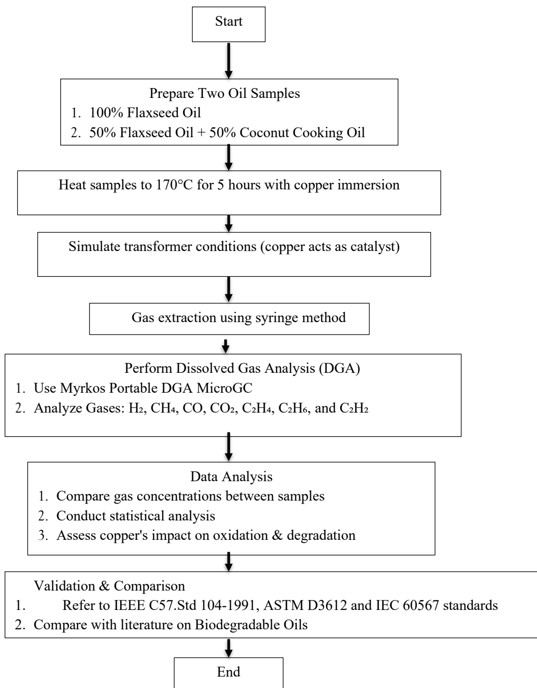
Figure 12. Flowchart
