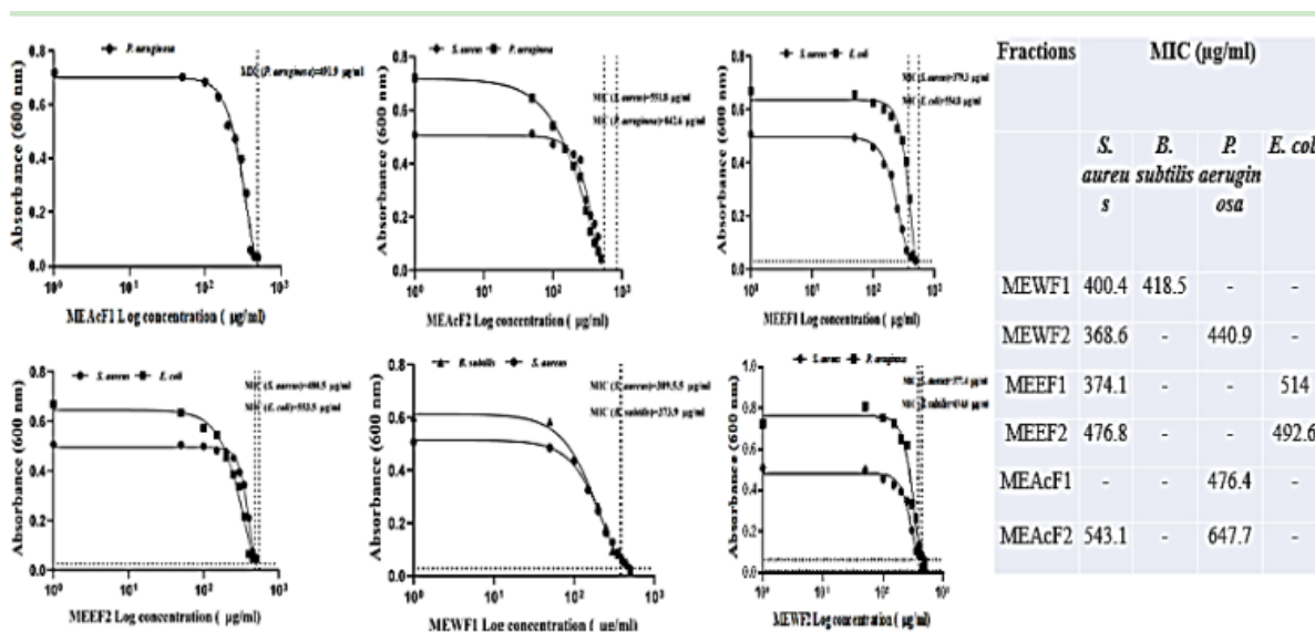
Figure 2: Determination of “Minimum Inhibitory Concentrations (MICs) of Extract Fractions Against Bacterial Strains. Dose response curves of MEAcF1, MEAcF2, MEEF1, MEEF2, MEWF1 and MEWF2 against Staphylococcus aureus , Bacillus subtilis , Pseudomonas aeruginosa , and Escherichia coli . The MIC values table, representing the lowest concentration at which bacterial growth was inhibited, is provided in the table.
