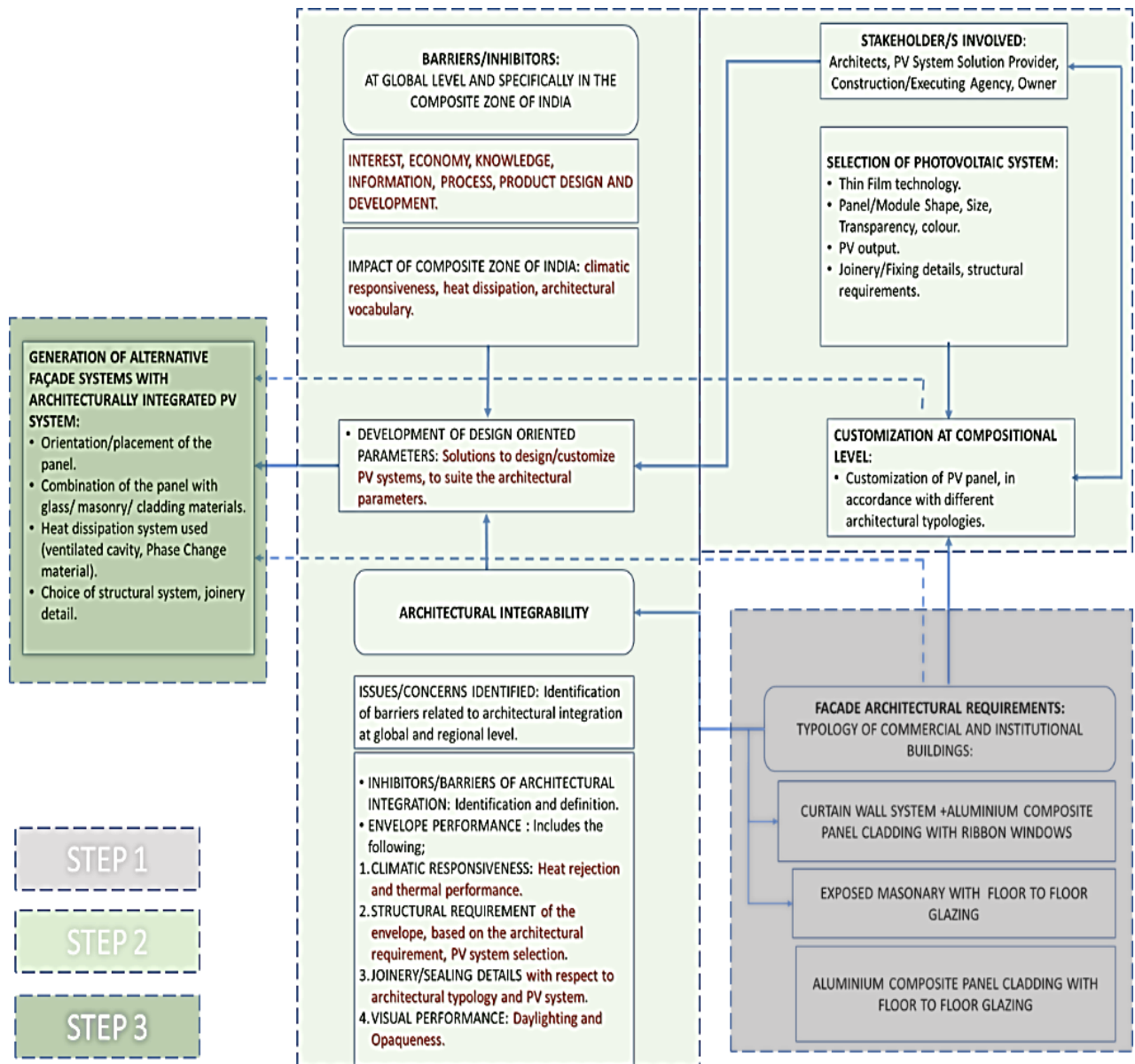
Figure 3: Framework for designing of photovoltaic facade and achieving architectural integration.
