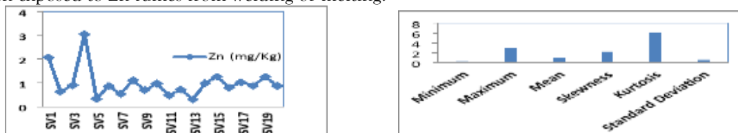
Figure 10: The Variation of Concentration of Zn (mg/kg) Present in Ladies Finger and Bar Diagram of Descriptive Statistics of Zn (mg/kg) Present in Ladies Finger
