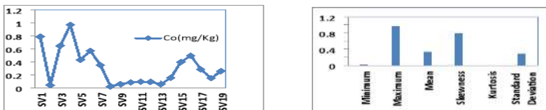
Figure 11: The Variation of Concentration of Co (mg/kg) Present in Raw Banana and Bar Diagram of Descriptive Statistics of Co (mg/kg) Present in Raw Banana
