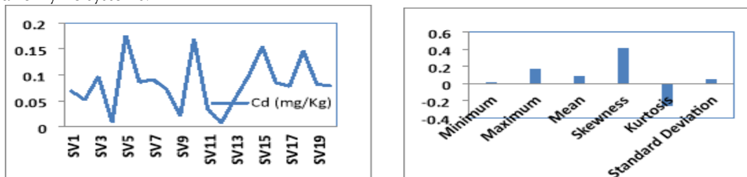
Fig.4: The Variation Pattern of Concentration of Cadmium in raw papaya and Bar Diagram of Descriptive Statistics of Cd (mg/Kg) in raw papaya
