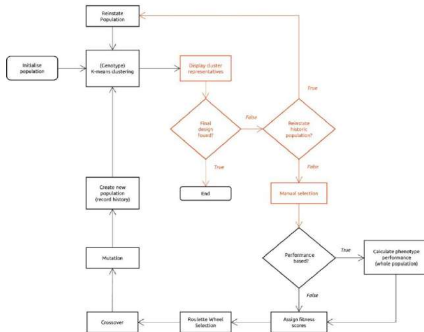
Figure 3: Developed by Harding J., 2018 in Biomorpher : Interactive evolution for parametric design, 2018
