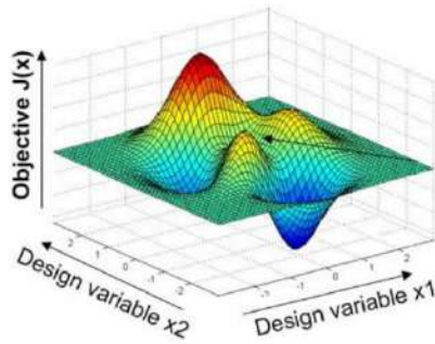
Figure 2: 3D Graph of an optimization problem, reproduced from Fasoulaki E., 2008 based on lecture notes of MITclass, ESD.77J Multidisciplinary system design.
