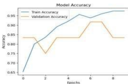
Fig. 5. Training and Validation Accuracy.
