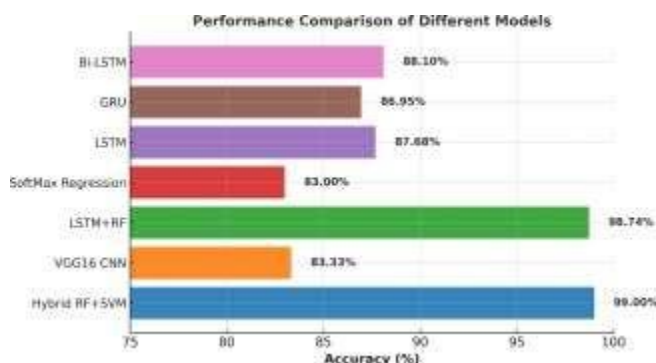
Fig. 4. Comparison of Classification Models.
