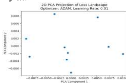
Figure 6. ADAM with 0.01 learning rate on the MNIST dataset.
