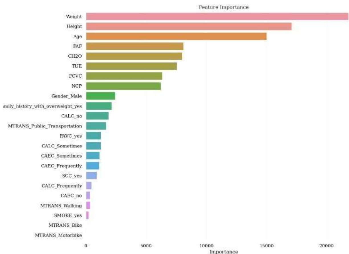
Figure 10: Important features selection
