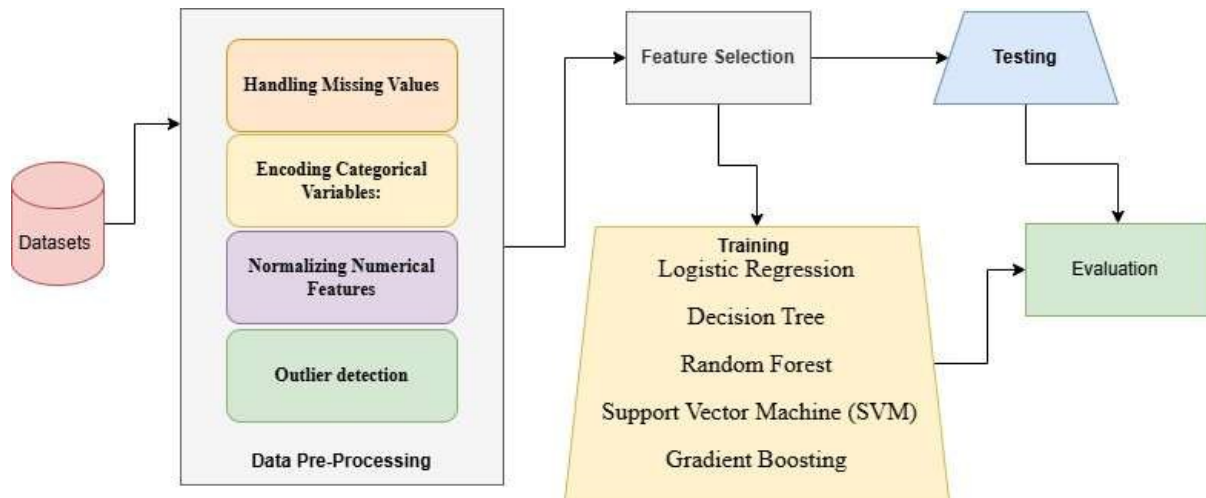
Figure 7: Block Diagram of proposed Model
