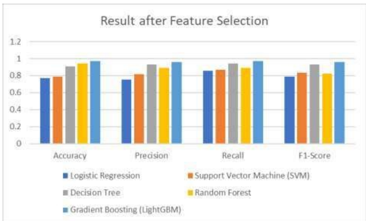
Figure 11: Result of different models after feature selection
