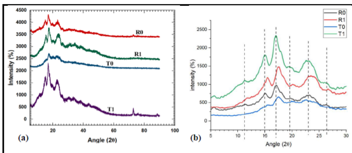
Fig. 3. The diffractogram of R_0 , R_1 , T_0 and T_1 starch (a), and the simulation of the main peaks (b) The graphs were separated on the vertical axis by 300 arb unit for better visualization.
