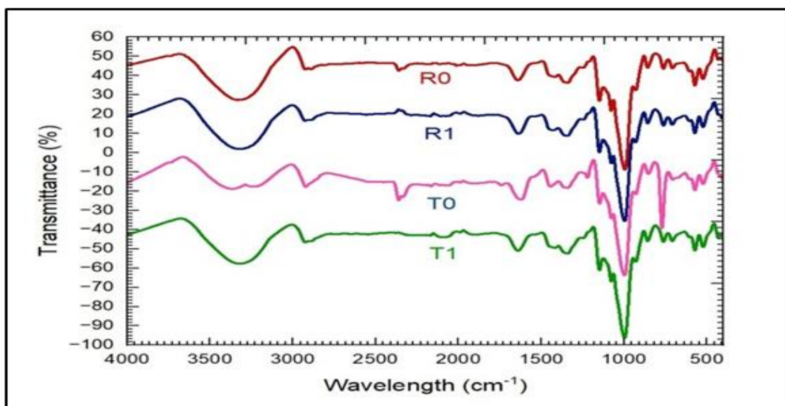
Fig. 1. FTIR combine spectra of native and gamma-irradiated starch
