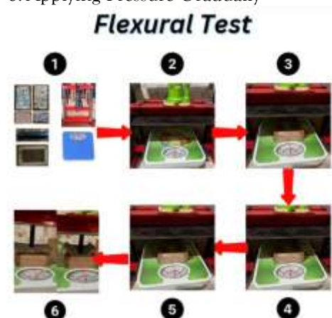
Figure 3.6 Testing Process
