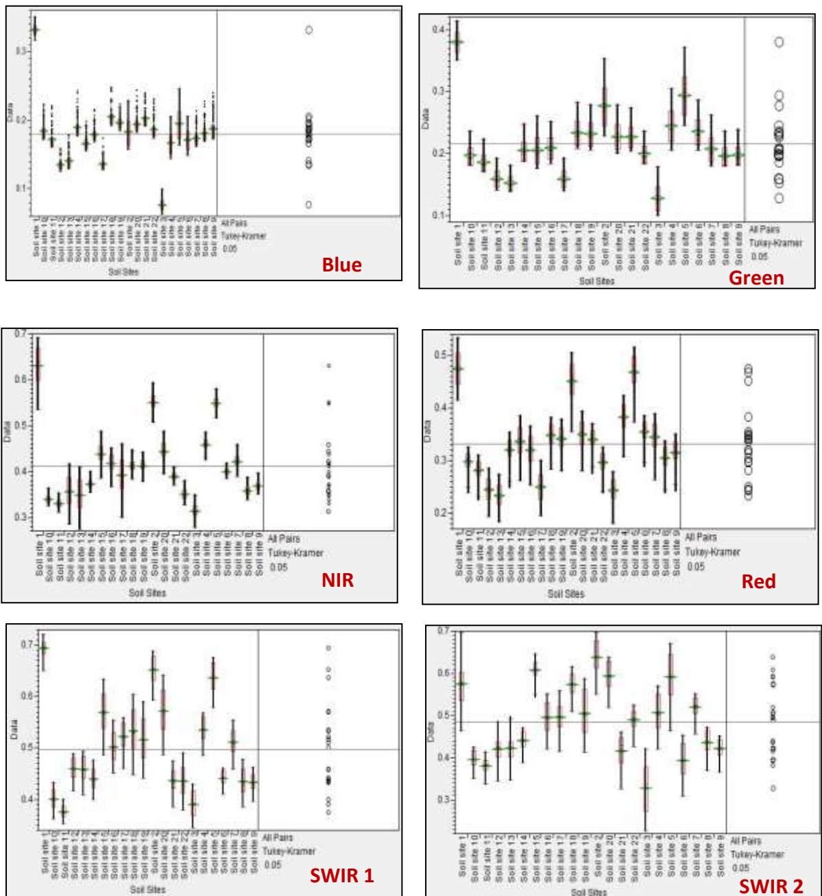
Fig.10. ANOVA and Tukey's HSD analysis of soil types across various spectral bands (Blue, Green, NIR and Red Zones, SWIRI and SWIRII).
