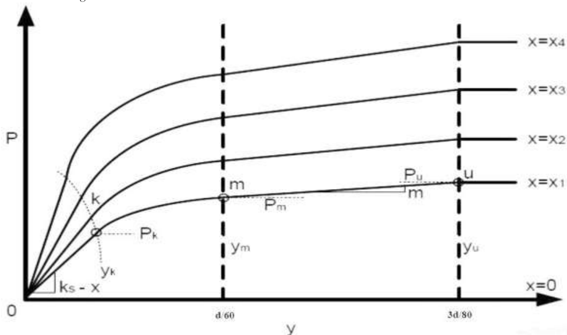
Fig.5 Construction of p-y curve
