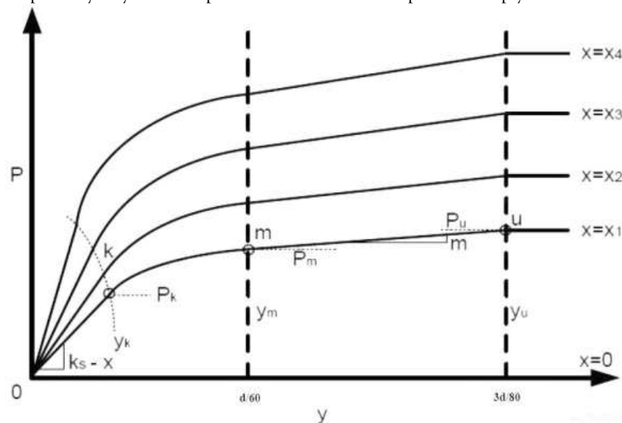
Fig.7 Characteristic shape of a family of p-y curve for static and cyclic loadings in cohesionless soil.
