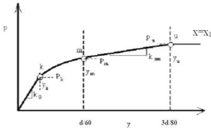
Fig.6 Construction of p-y curve
