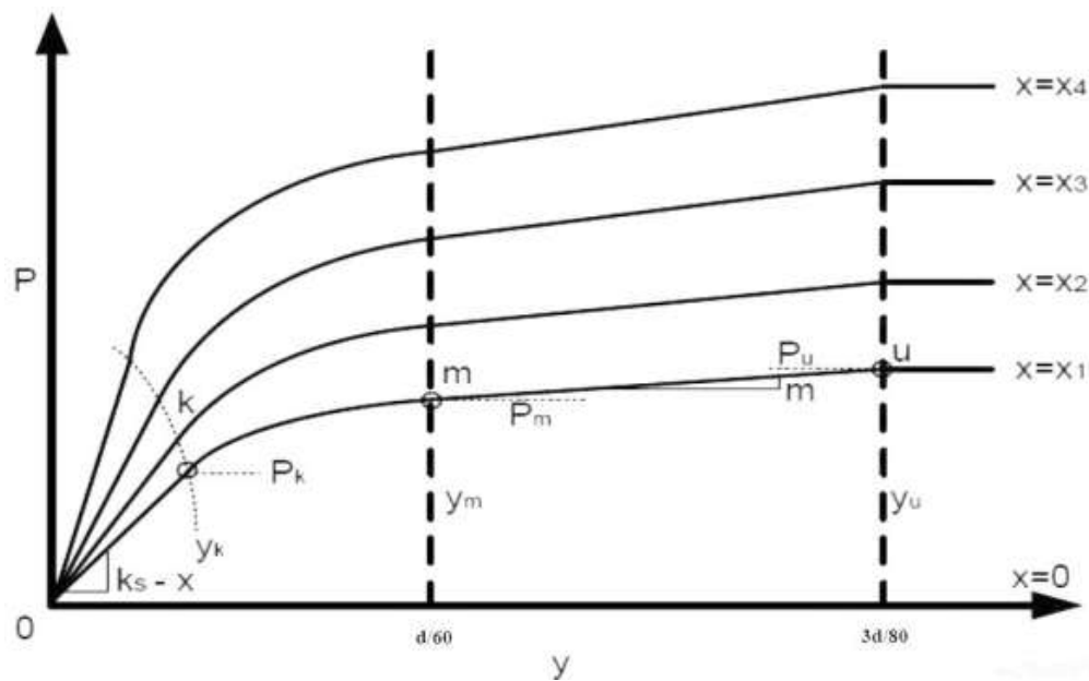
Fig.1(c) Characteristic shape of a family of p-y curves for static and cyclic loading in cohesionless soil While neither of these conditions is precisely met in practice. It is believed that in most instances the assumptions can be made without serious error. The deformation of the pile through a distance y_1 as shown in Fig.1(c), would generate unbalanced soil pressures against the pile, perhaps as indicated in the figure. Integration of the soil pressures around the pile would yield an unbalanced force p_1 per unit of length of the pile.
