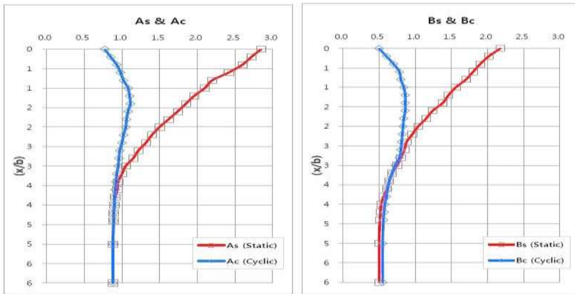
Fig.8 Values of coefficients A_s and A_c .
