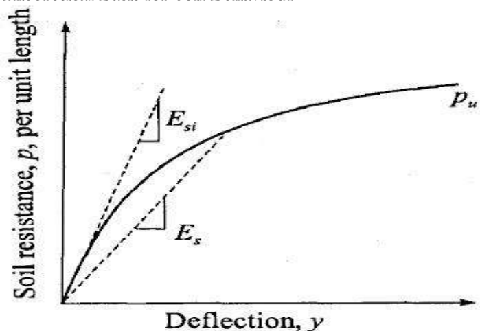
Fig.3 Characteristic shape of a p - y curve
