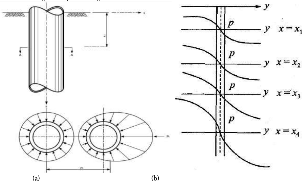
Fig.1(a) Definition of soil response curve,
