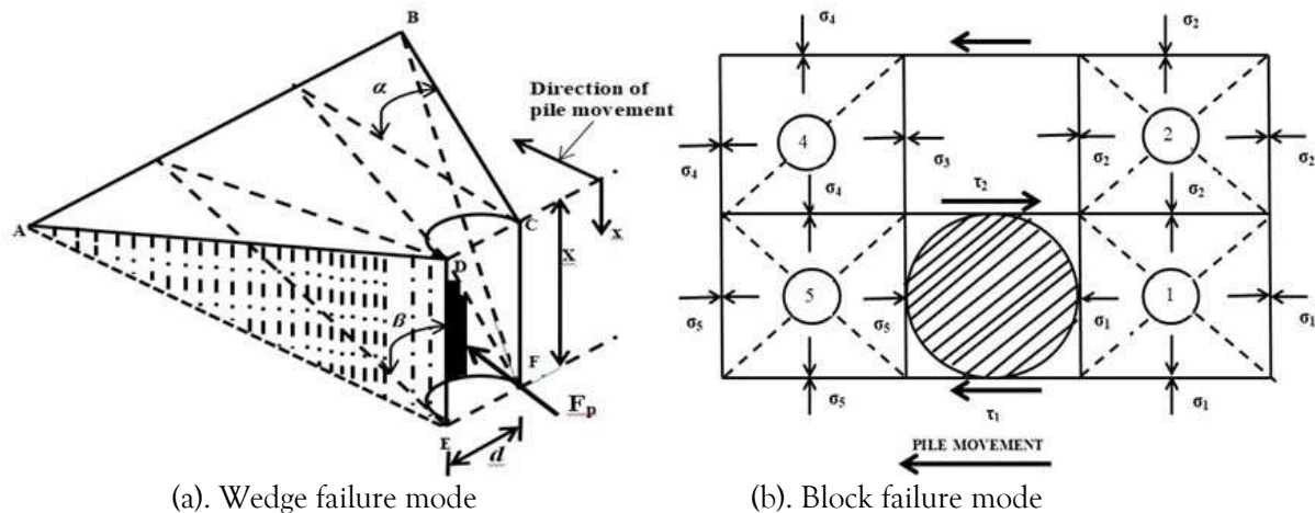
Fig.4 Two types of soil failure mode
