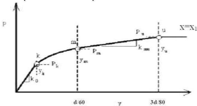
Fig.2 Construction of p-y curve
