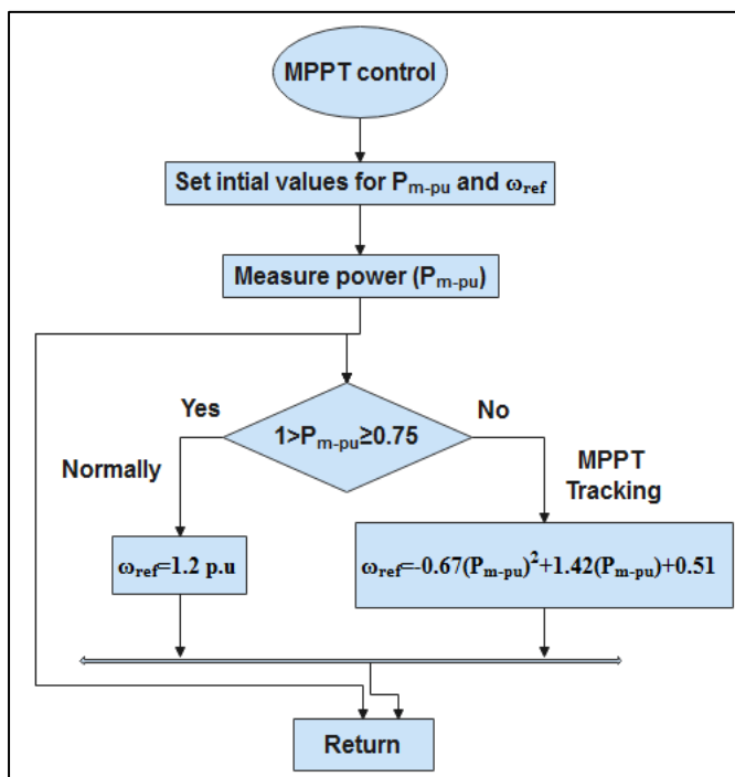
Figure 4. Improved MPPT Strategy Flowchart Incorporating Mechanical Power Analysis
