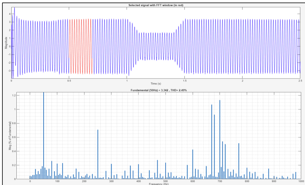
Figure 8(e). THD with FLC Controller
