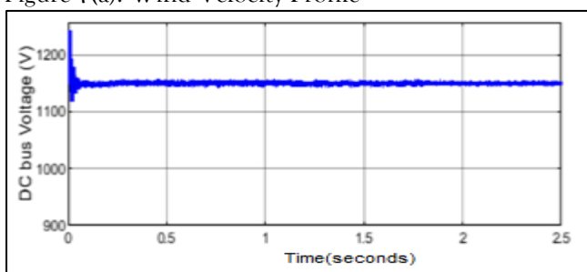
Figure 7(b). DC-Link Voltage(Vdc) of DFIG
