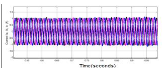
Figure 7(e). Wind Farm-Injected Current
