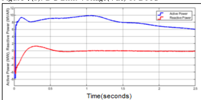
Figure 7(c). Injected P and Q from Wind Farm
