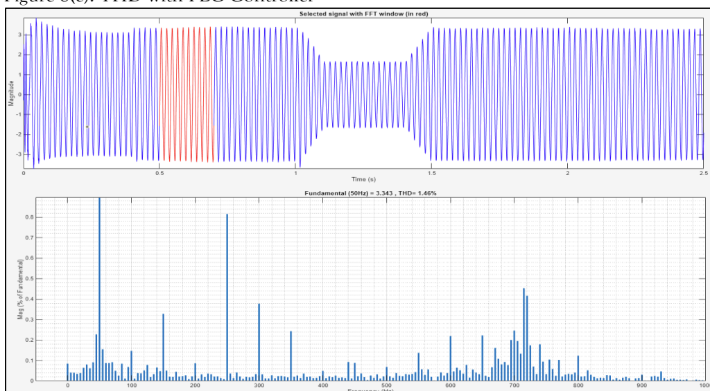
Figure 8(f). THD with PI Controller
