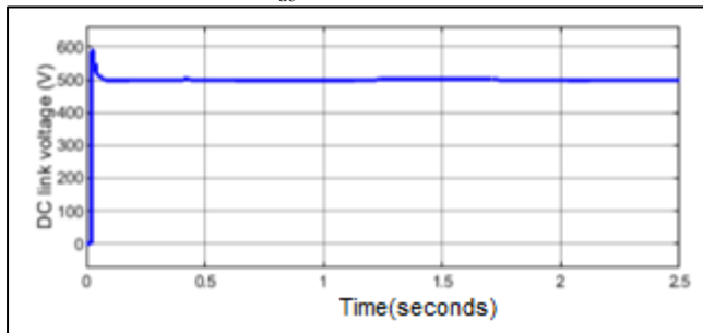
Figure 6(b). DC Link Voltage Management with ANN Controller
