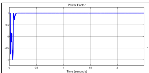
Figure 5(g). PFC of the Inverter using PI
