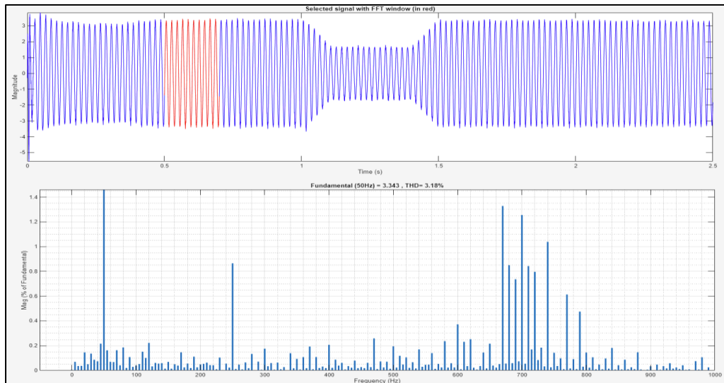
Figure 8(d). THD with PI Controller
