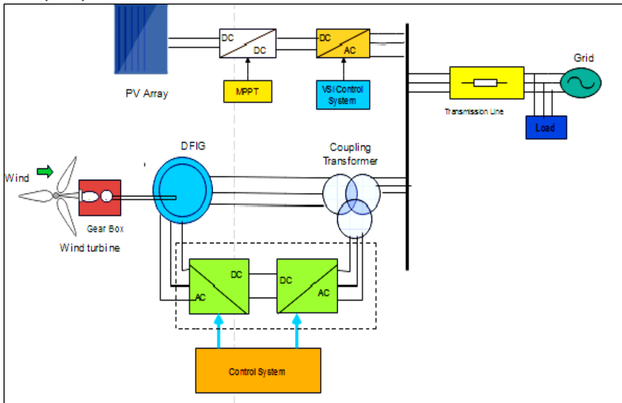
Figure 1 Renewables Integration Designing Solar-Wind Systems
