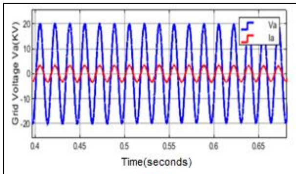
Figure 5(e). 3- \Phi V-I Waveforms Controlled by PI
