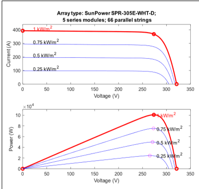
Figure 2. Performance Traits of PV Arrays across Changing Solar Irradiance
