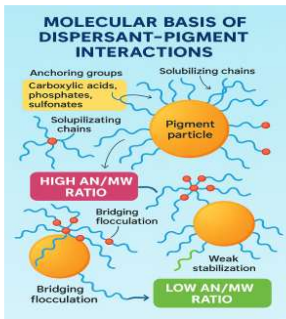
Figure 1: Molecular interactions between dispersant molecules and pigment particles
