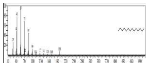
Tetradecane
