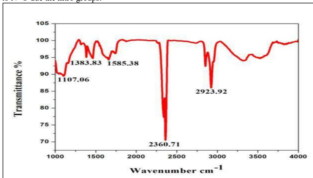
Figure 3: FT-IR spectrum of the synthesized AgNPs using the leaves extract of Acalypha indica.L . Antibacterial assay of Plant Extract shown Potential activity against experienced human pathogenic organism. The green way synthesized good activity against all pathogenic range.
