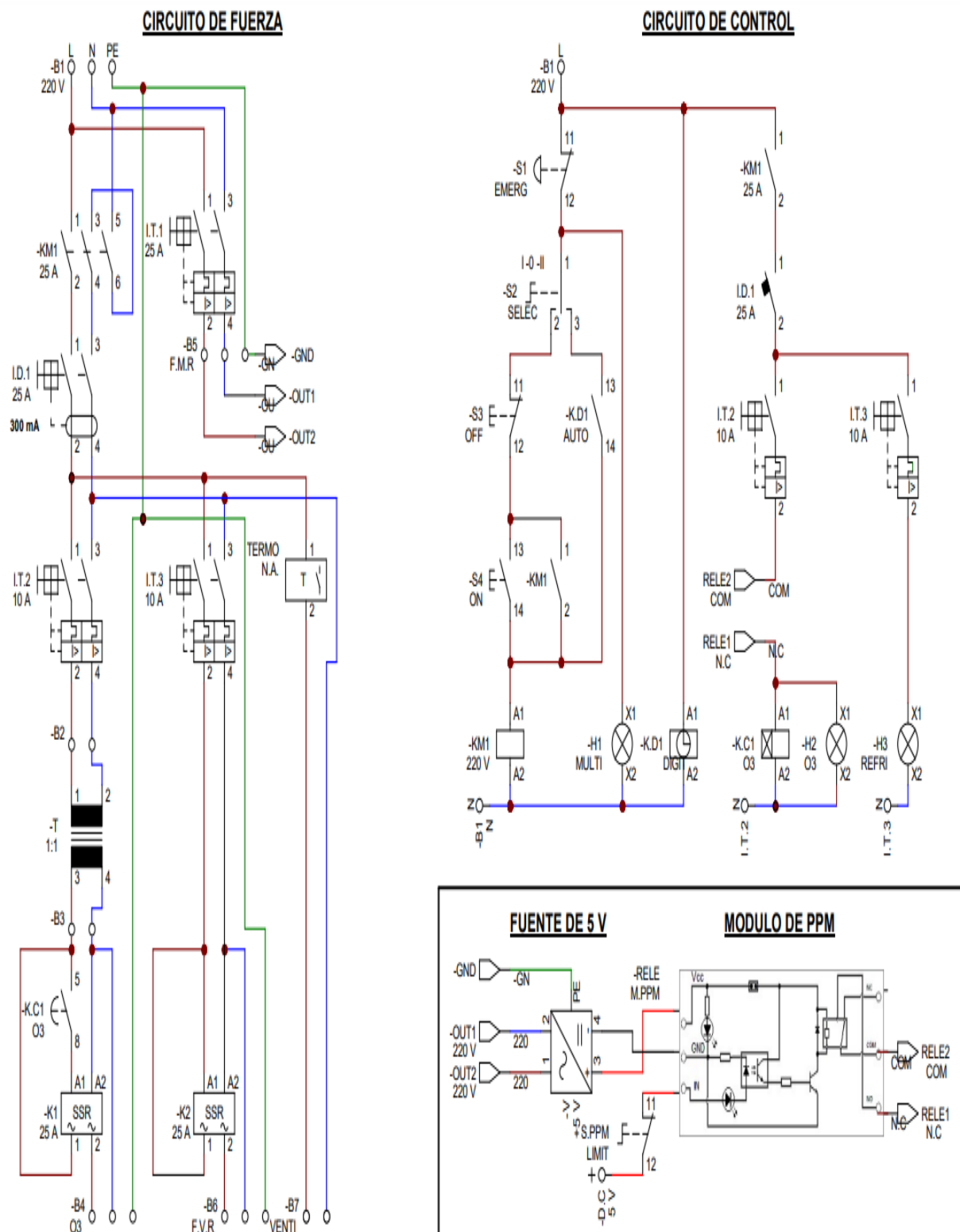
Figure 1 Electrical Circuit
