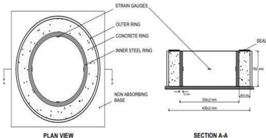
Figure 1: schematic of ring specimen
