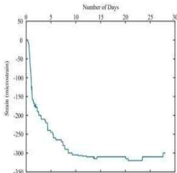
Figure 4: strain vs. time for M40 concrete
