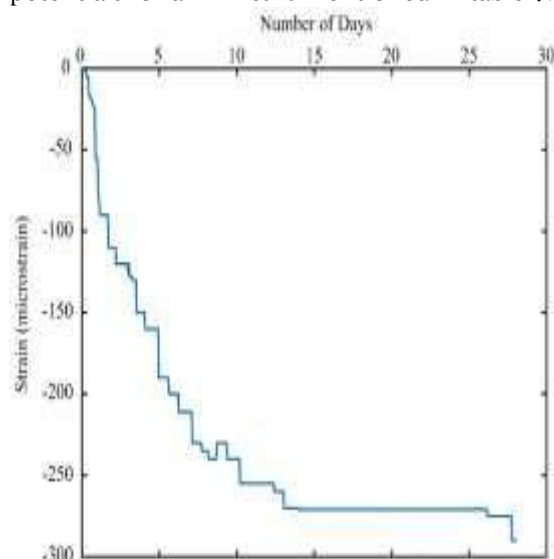
Figure 3: strain vs. time for M20 concrete
