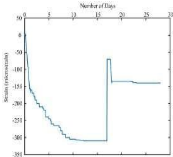
Figure 5: strain vs. time for M60 concrete
