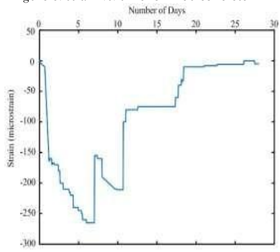
Figure 8: strain vs. time for M120 concrete
