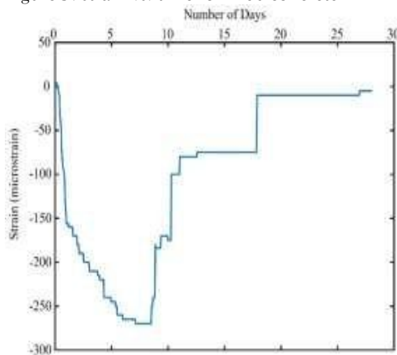
Figure 7: strain vs. time for M100 concrete
