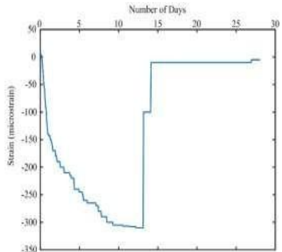
Figure 6: strain vs. time for M80 concrete
