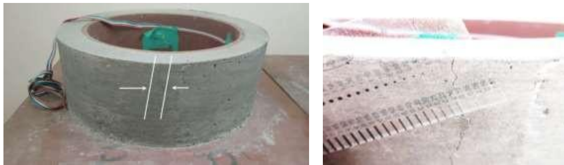
Figure 10 (a): M80 moulded concrete Figure 10 (b): Photo showing crack and crack width measurement
