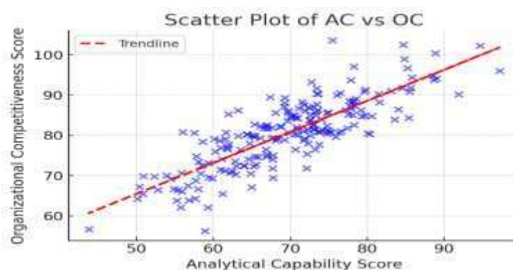
Figure 3: Scatter Plot of AC vs OC
