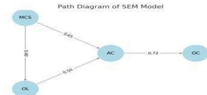
Figure 2: Path Diagram of SEM Model
