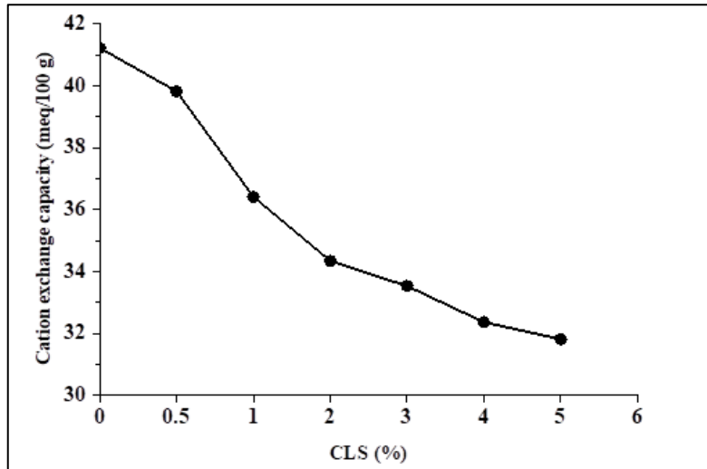
Figure 8: Effect of CLS on CEC of BC soils.
