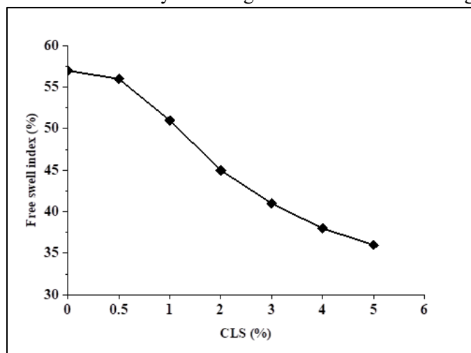
Figure 4: Effect of CLS on FSI
