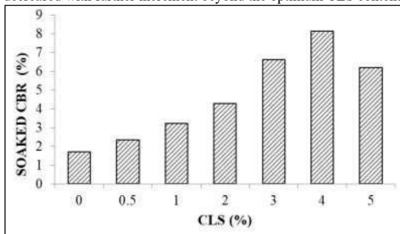
Figure 7: Effect of CLS on Soaked CBR
