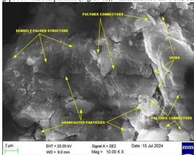
Figure 12: FESEM micrograph of CLS treated BC soil
