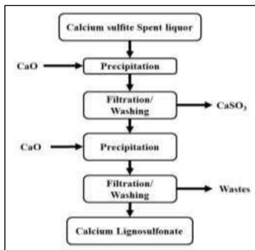
Figure 2: Schematic separation of calcium lignosulfonates from calcium sulphite wasted liquor.
