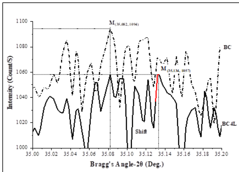
Figure 10: Reduction and shifting of the M-peak strength of untreated and treated BC soil ‘
