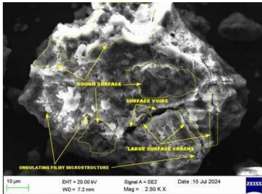
Figure 11: FESEM micrograph of BC soil
