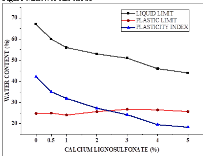
Figure 5: Effect of CLS on Plasticity characteristics
