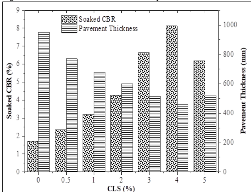
Figure 14: Effect of Soaked CBR on Pavement Thickness
