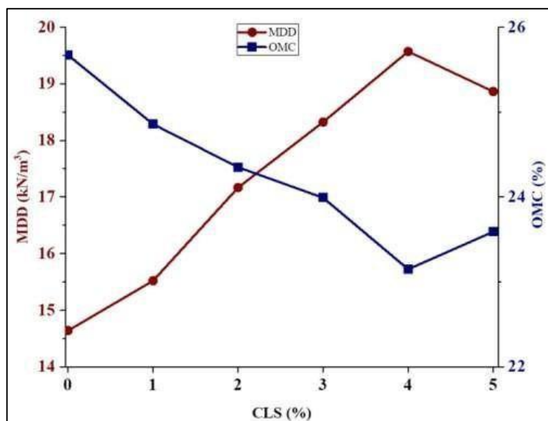
Figure 6: Compaction characteristics of treated BC soil
