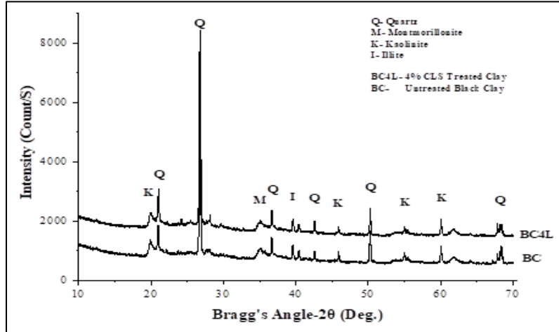
Figure 9: Comparison of the XRD patterns of BC soil and 4% CLS treated BC soil
