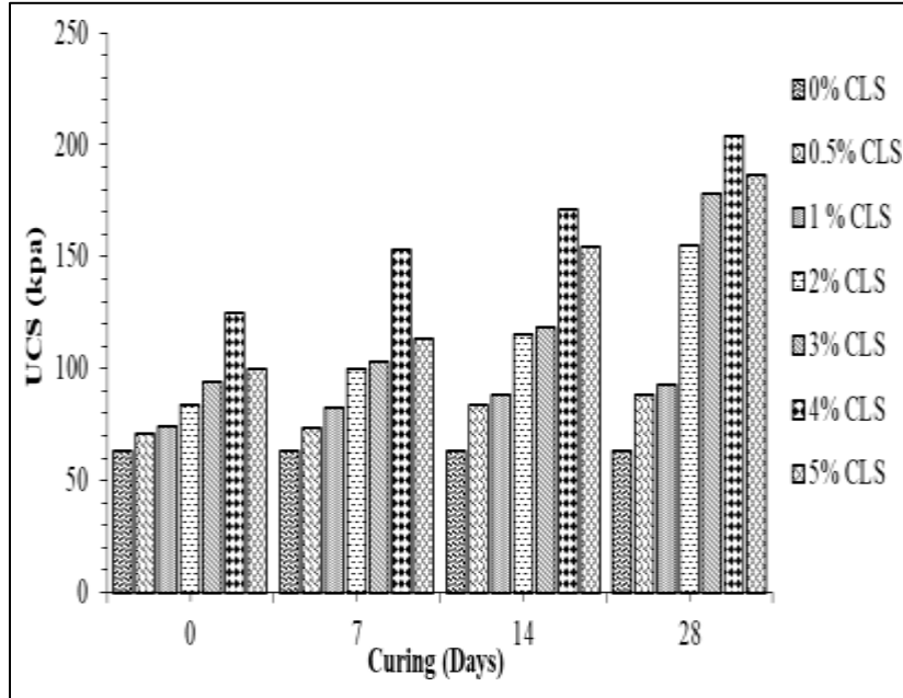
Figure 13: UCS of CLS-treated BC soil samples
